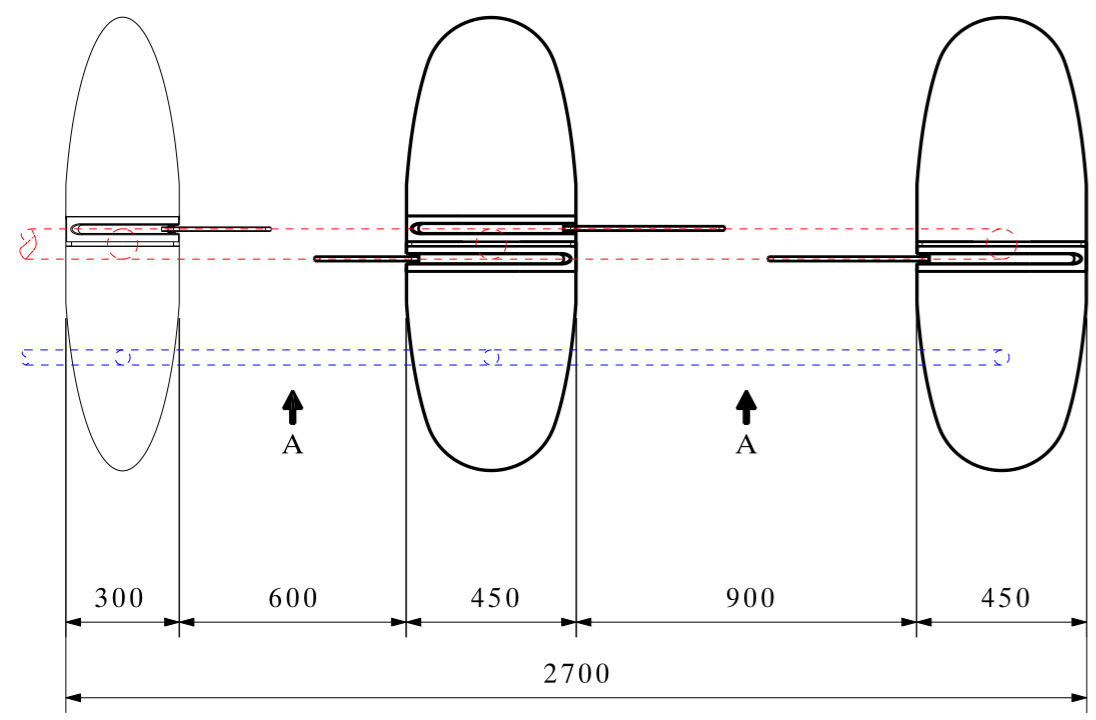
LEFT-HAND GATE SL900 INTERMEDIATE(HYBRID) GATE SL910 RIGHT-HAND GATE SL910
