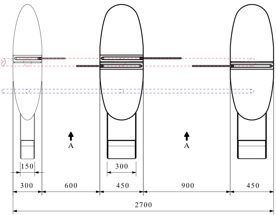
LEFT-HAND GATE SL901 INTERMEDIATE(HYBRID) GATE SL911 RIGHT-HAND GATE SL911
