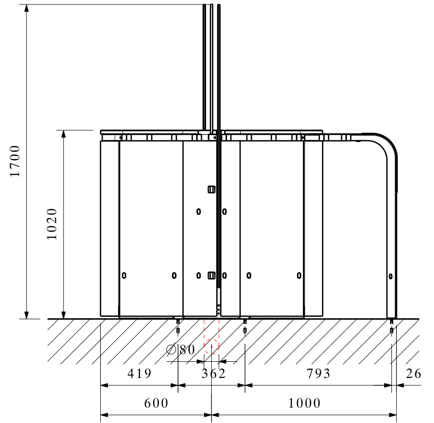
VIEW Y-Y
