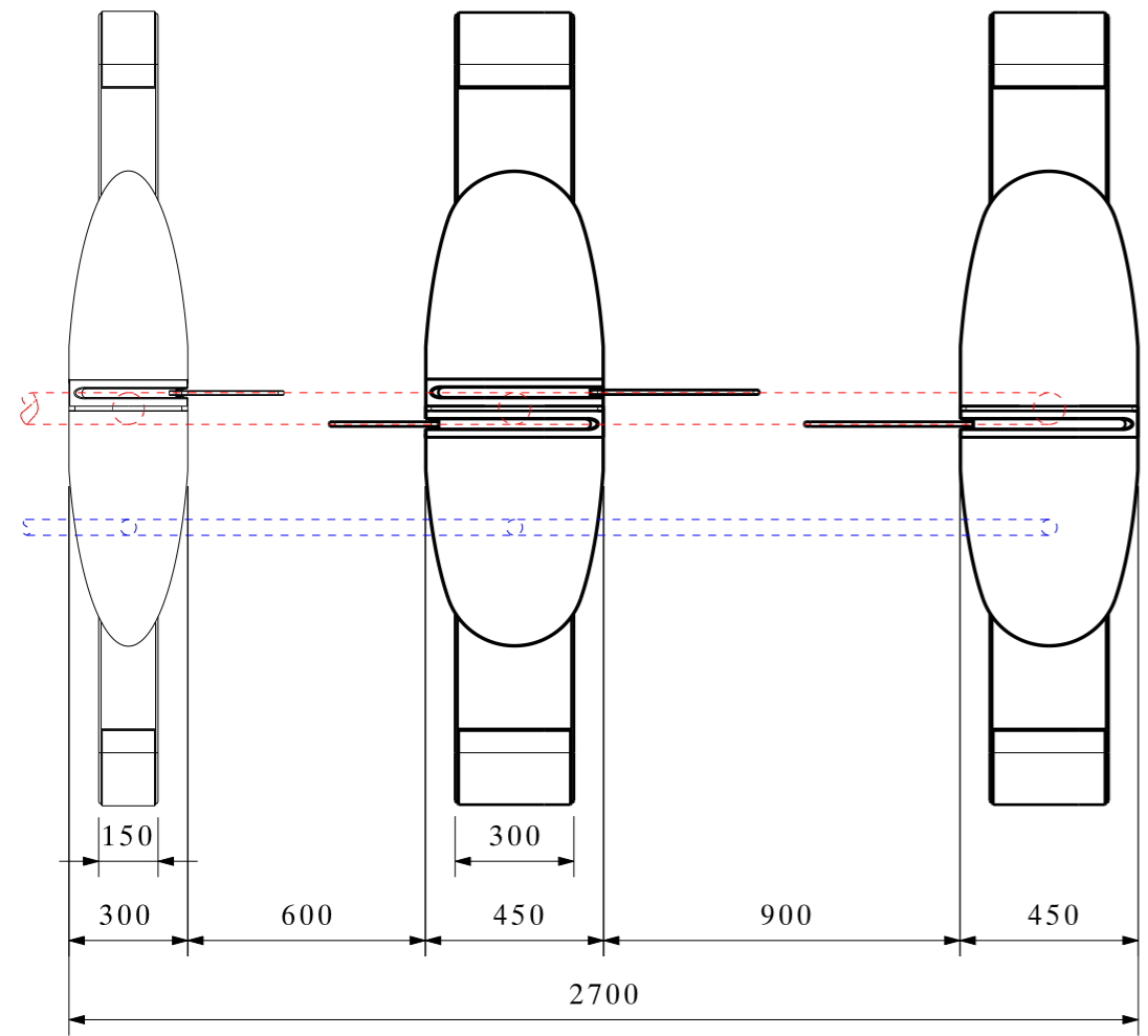
LEFT-HAND GATE SL902 INTERMEDIATE(HYBRID) GATE SL912 RIGHT-HAND GATE SL912
